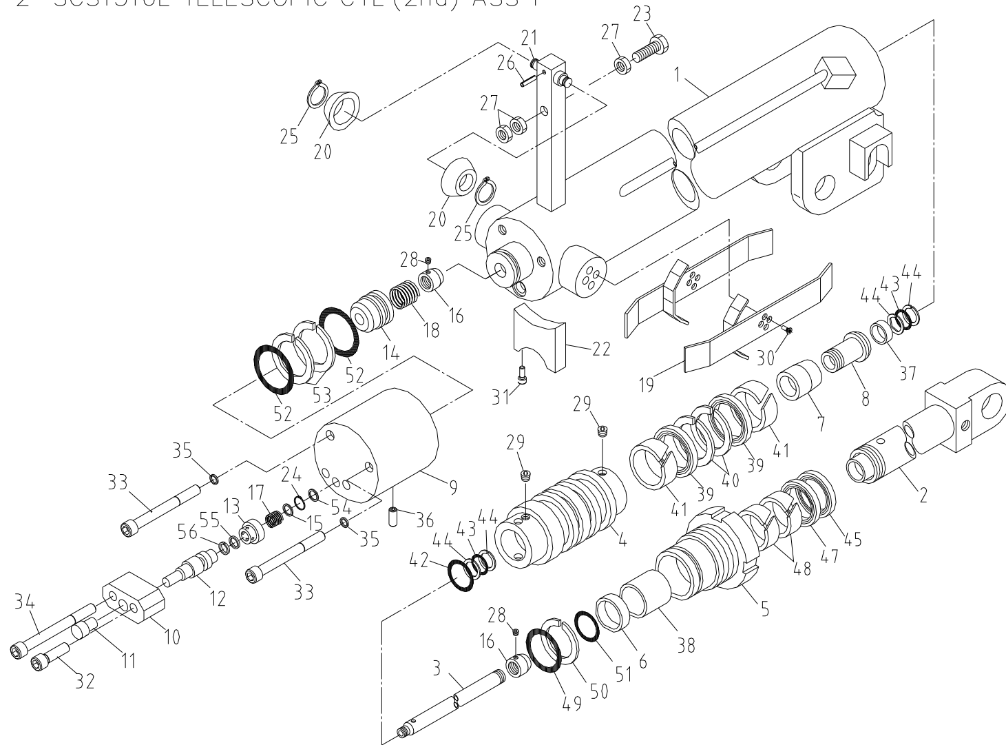
Fig. 1-1-2 SCS1516L TELESCOPIC CYL'(2nd) ASS'Y
