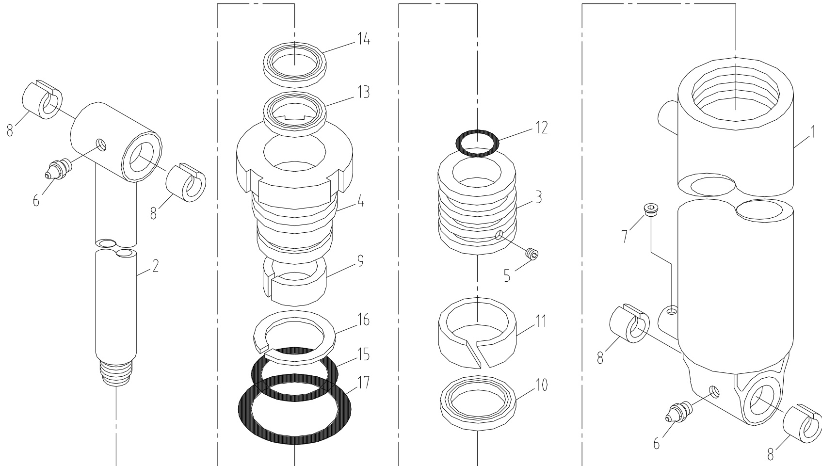
Fig. 2-1 SCS1516L DERRICK CYL' ASS'Y
