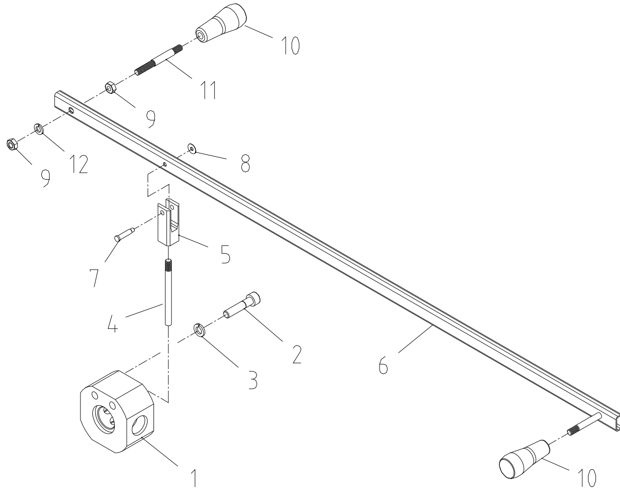
Fig. 3-1 SCS1516L DIVERter V/V SET
