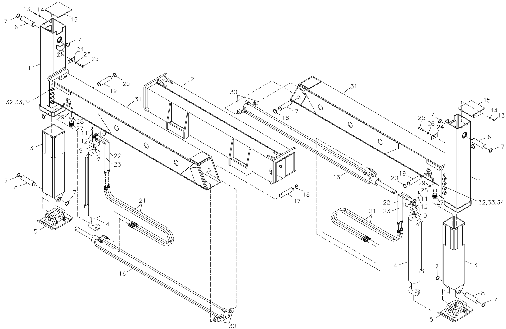
Fig. 9-2-1 SCS1516L REAR OUTRIGGER ASS'Y
