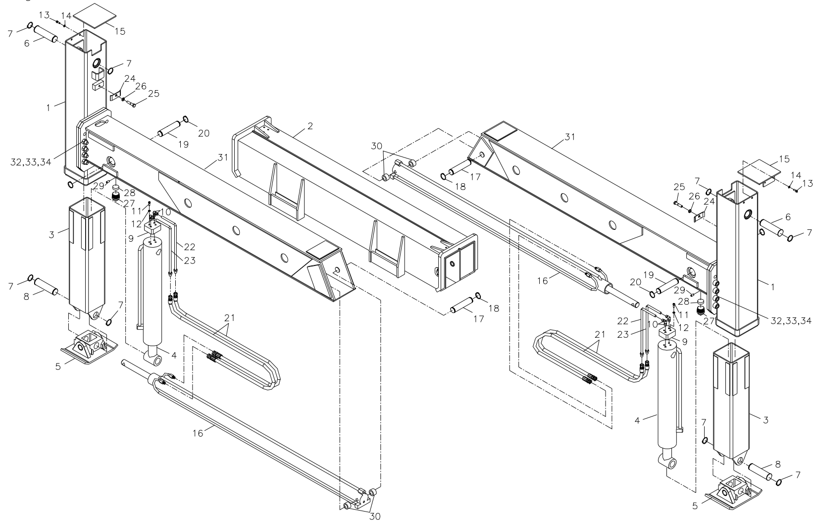
Fig. 9-2-1 SCS1516L REAR OUTRIGGER ASS'Y
